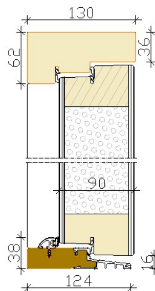
Combi threshold
