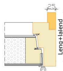
Jamb with extension
