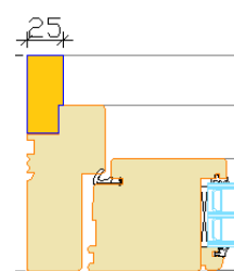
Jamb with extension
