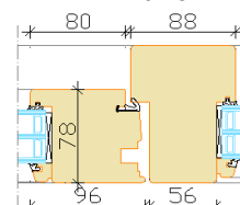
Mullion
