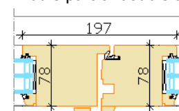
Middle part of double door
