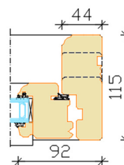
Openable window
