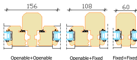
Openable+Openable
