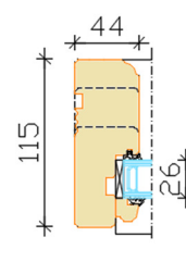
Fixed window
